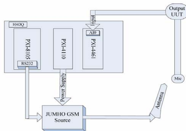
Hardware connect diagram
